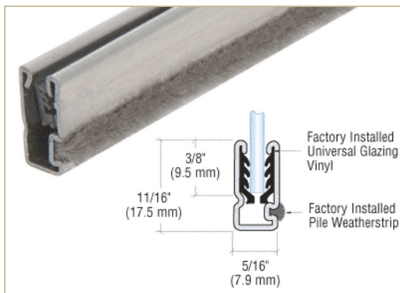
Detail of storm panel frame
