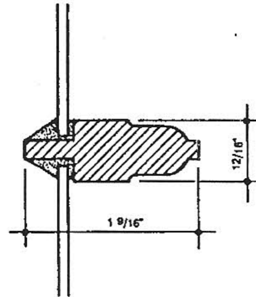
1870s WOOD MUNTIN
