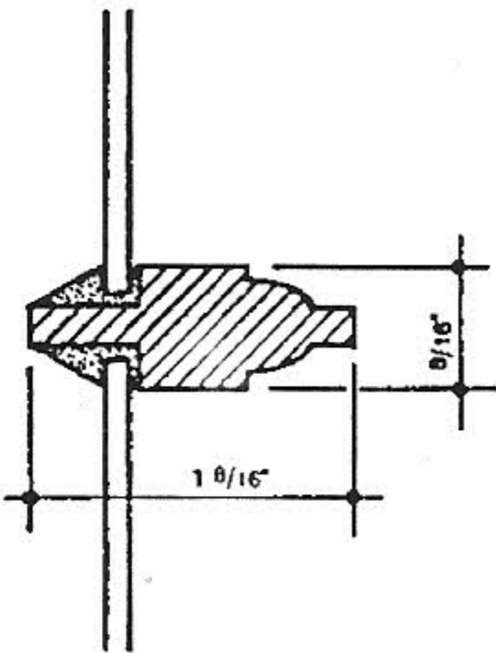
1845 WOOD MUNTIN
