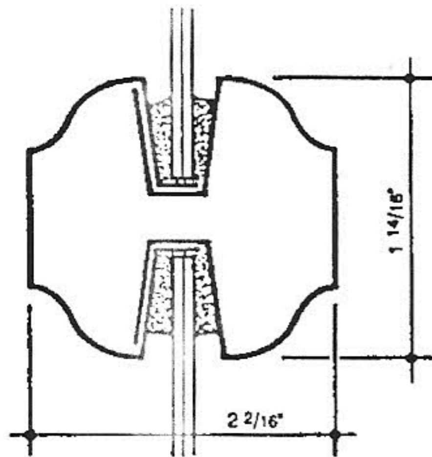
1905 HOLLOW-CORE METAL MUNTIN
