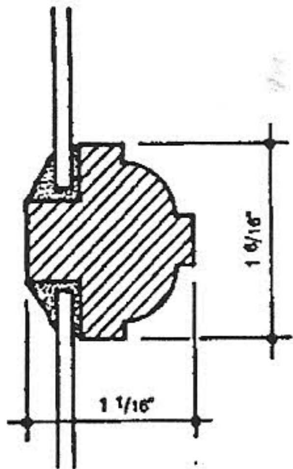
1740s WOOD MUNTIN
