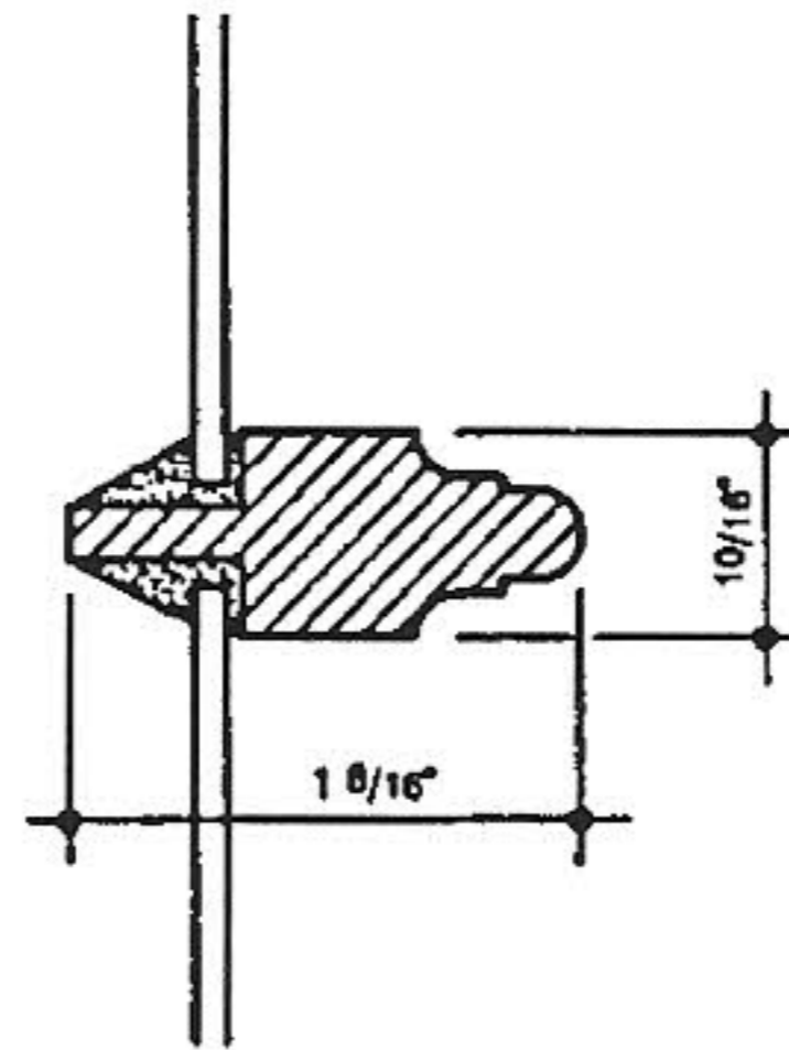
1823s WOOD MUNTIN
