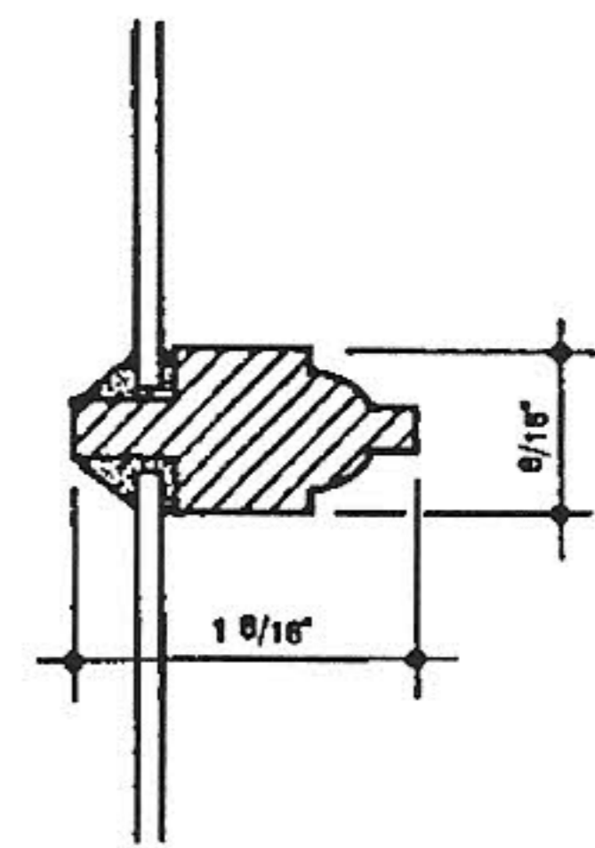
1835s WOOD MUNTIN
