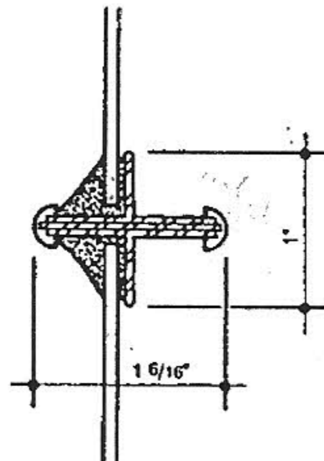
1911 STEEL MUNTIN
