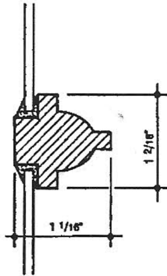
1760s WOOD MUNTIN
