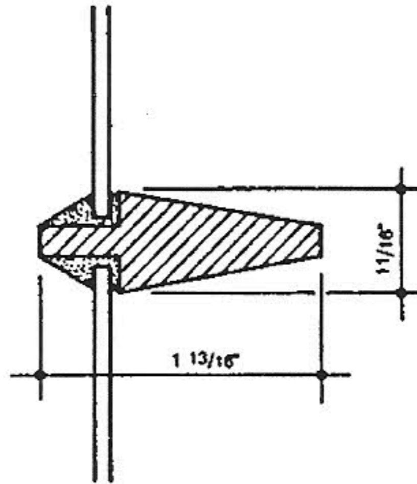
1850s WOOD MUNTIN
