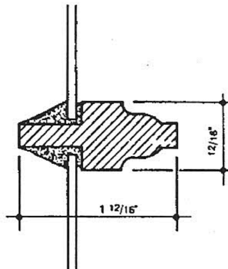
1915 WOOD MUNTIN
