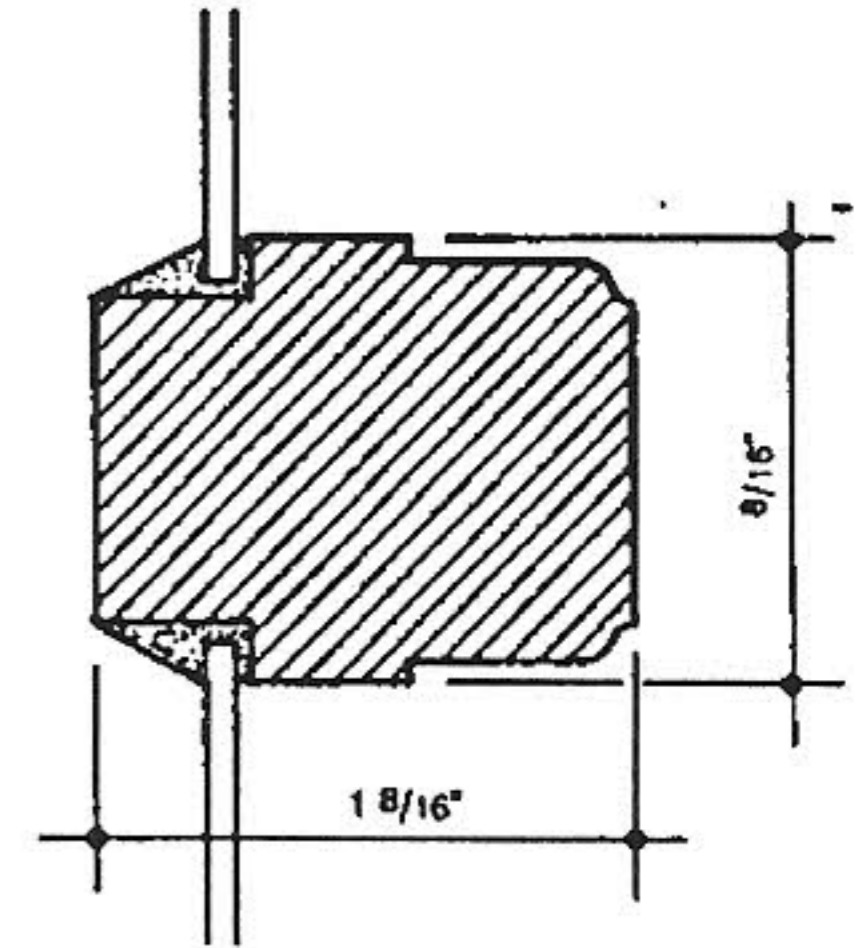
1879 WOOD MUNTIN
