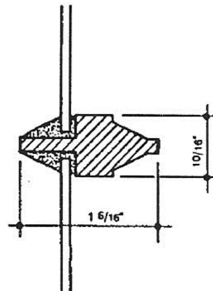
1932 WOOD MUNTIN
